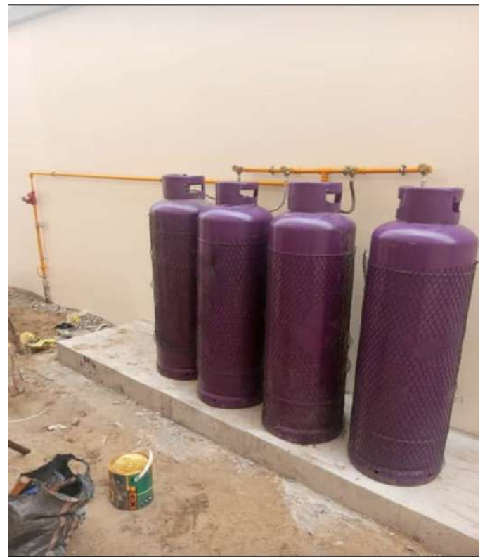
Ongoing Gas Cylinder Manifold Installation
